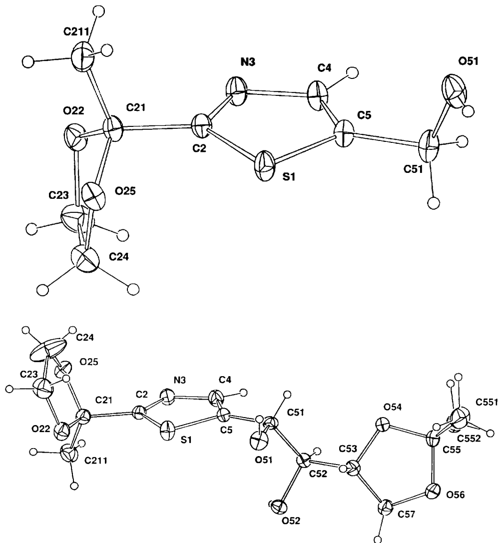
Figure 1. Projection of 6 (top structure) and 13 (bottom structure); 20% thermal ellipsoids are shown for the non-hydrogen atoms, hydrogen atoms having arbitrary radii of 0.1 Å. Note that the ellipsoid in 13 for C(24), possibly a foil for unresolved disorder, is suggestive of a pair of alternative ring configurations superimposed.
